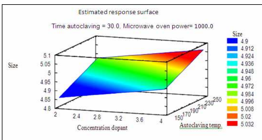
Figure 5. Estimated response surface (concentration dopant – autoclaving temperature)
