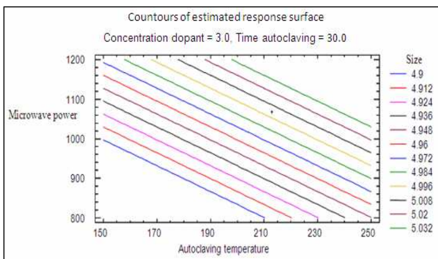
Figure 14. Contours of estimated response surface (autoclaving temperature – microwave power)
