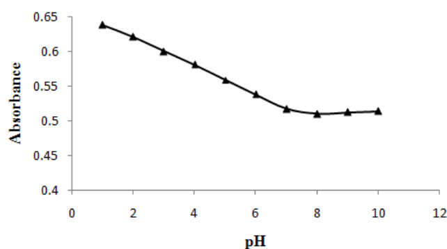
Figure 2. Effect of pH on absorbance. [\text{Mo(VI)}] = 4 \times 10^{-6} M; [\text{SAAH}] = 4 \times 10^{-5} M
