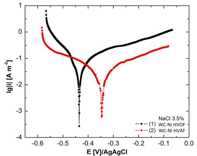
Figure 5. Polarization curves of WC-Ni coatings
